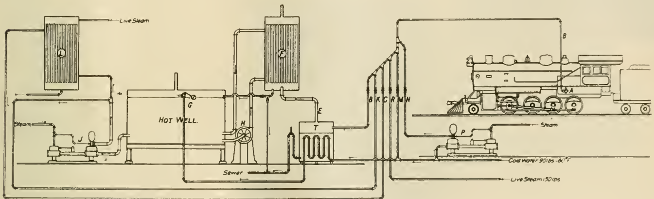
FIG. 4. DIAGRAM OF WATER CHANGING APPARATUS, P. & L. E. RAILROAD, MCKEES ROCKS SHOPS.
